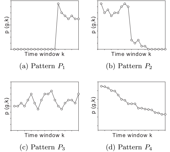
Figure 4: Representative Time Series Patterns for Groups
