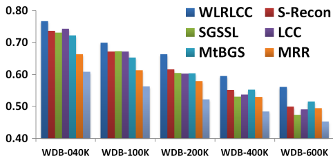
Fig. 6. Comparison between WLRLCC and the other algorithms on WDB-040K, WDB-100K, WDB-200K, WDB-400K, and WDB-600K
