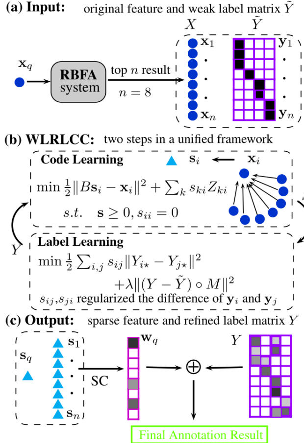
Fig. 2. Illustration of the proposed WRLCC process. In this example, we show the top n = 8 retrieved images with m = 4 candidate names for query image \mathbf{x}_q : (a) gives the input data; (b) illustrates the two key steps of the WRLCC process; (c) shows the output coding result and final annotation scheme.
